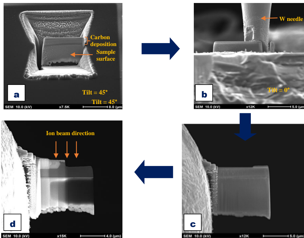
Figure 3. SEM images: (a) specimen coated and dug until 1 \mu m slice remains, (b) slice removed using needle, (c) slice attached to TEM mesh, (d) specimen thinning (15 kV to 3 kV accelerating voltage).
